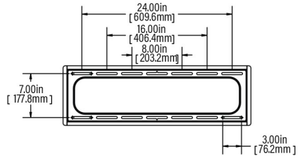
WALL PLATE
