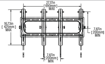
WALL PLATE
