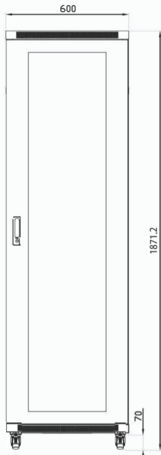
FRONT VIEW
