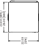
top sectional view of PTRK side
