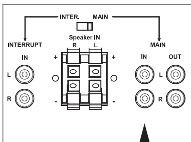
Use these Inputs to connect Pre-amp or Receiver Line Out
