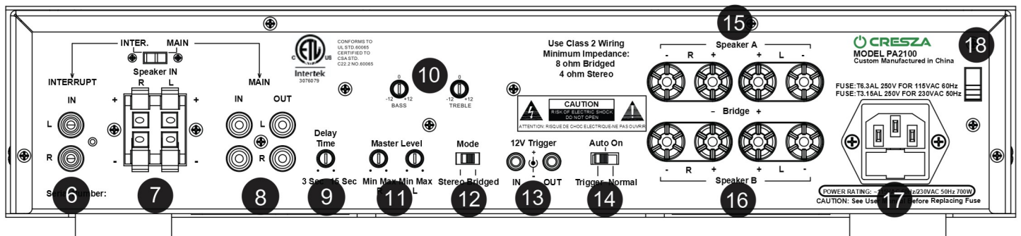
Figure 2. Rear Panel
