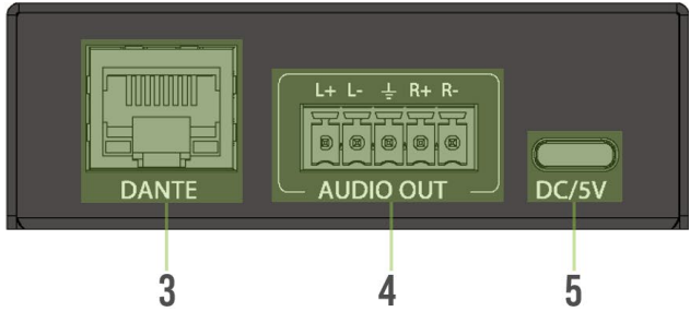
Rear Panel
